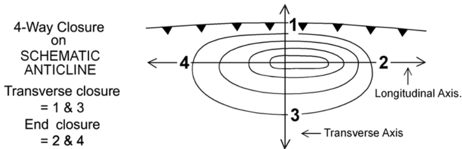
Figure 12. Anticlines must have closure on all sides ("4-way closure") in order to trap oil, and most anticlines do, indeed, have 4-way closure unless they are later tilted.
