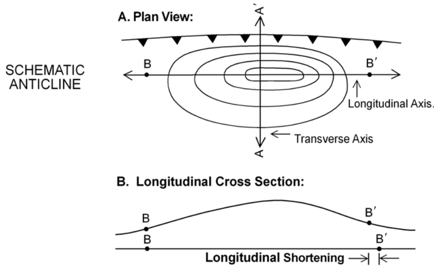
Figure 13. This simple longitudinal cross-section shows that longitudinal shortening does exist.
