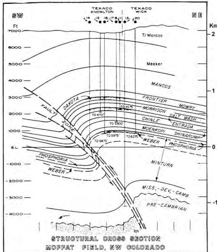
Figure 6. Don Stone, Denver geologist, favored a model similar to Bob Berg's in this 1975 cross-section. Note down-plunging fault zone.
